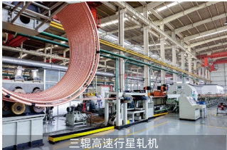
HIGH-SPEED PLANETARY MILLING MACHINERY
